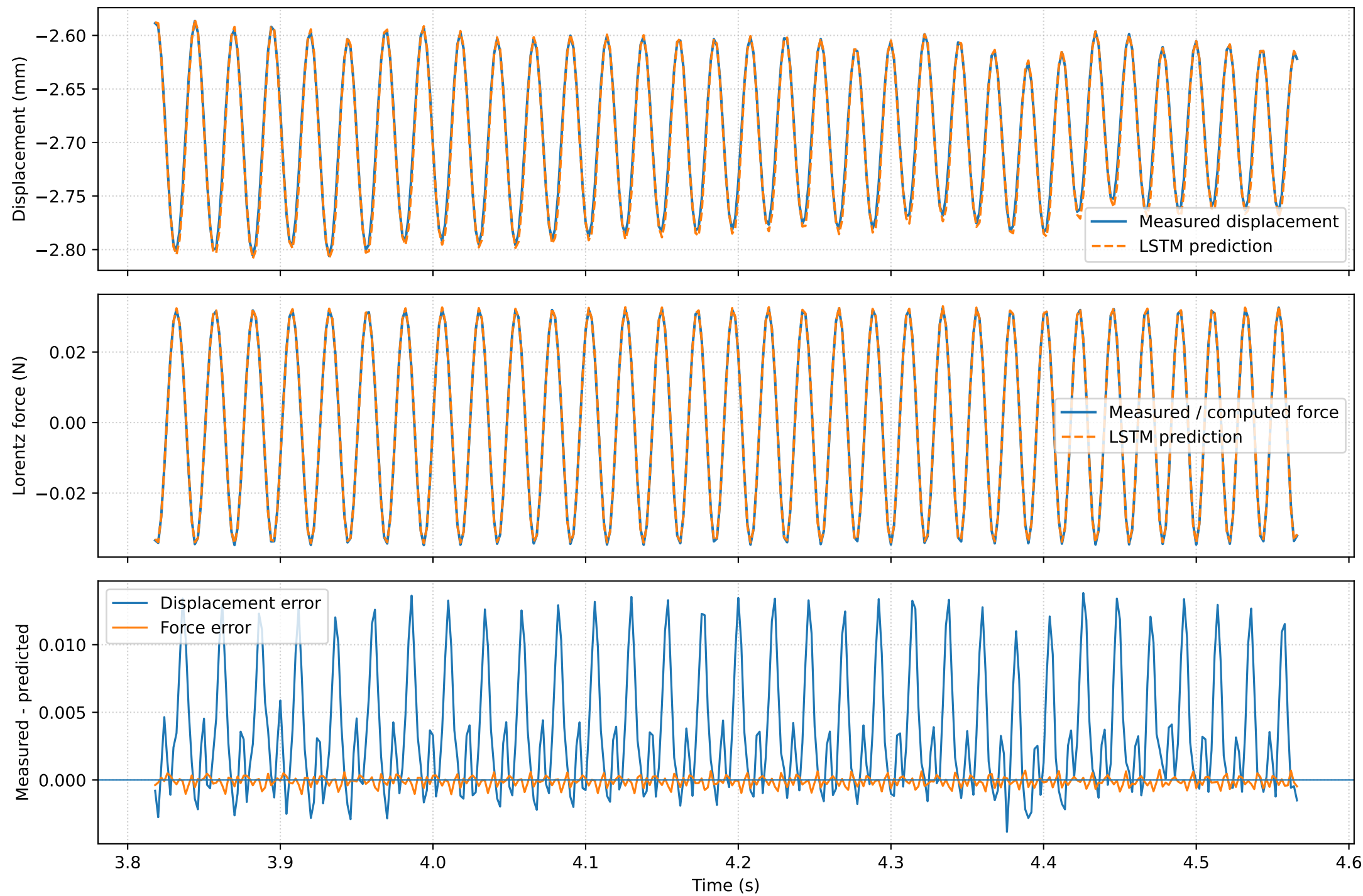
Zoomed LSTM tracking: Chirp_1 | center = 4.192 s | window = 0.750 s
